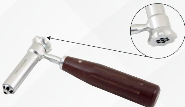
812.020 Protection Sleeve for Suprapatellar Tibia Nail
